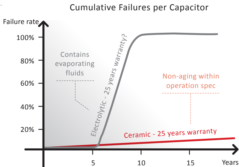
Figure 4: Ceramic capacitors have a significantly longer lifetime than electrolytic capacitors.
